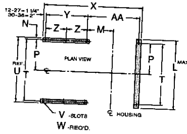
Principal Dimensions (Inches) – Sizes 12" – 36"
