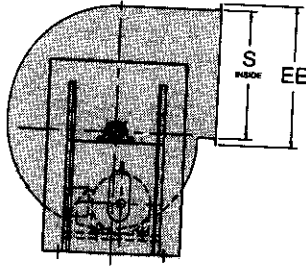
Principal Dimensions (Inches) – Sizes 12" – 36"
