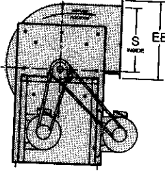
Principal Dimensions (Inches) – Sizes 12" – 36"
