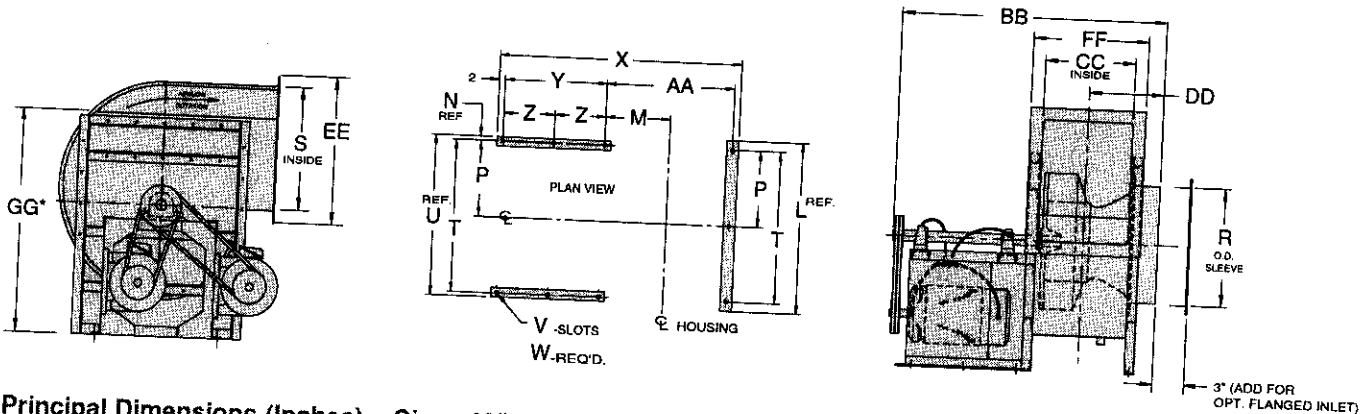
Principal Dimensions (Inches) – Sizes 40" – 60"
