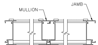
PLAN VIEW SCALE: 1-1/2" = 1'
