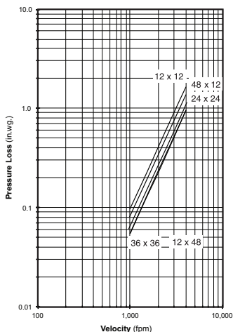
Figure 5.2 — Ducted Inlet
