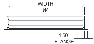
MODEL: 2635DC FRAME: FLANGE FRAME FLANGE-MOUNT (FM)
