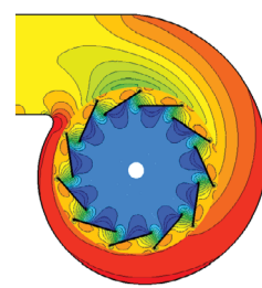
Pressure Contours (Centrifugal fan)
