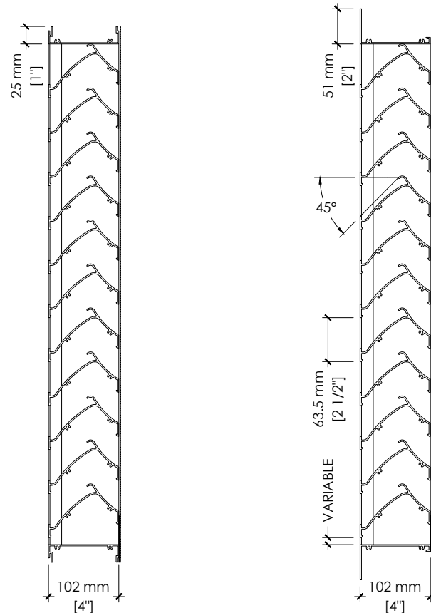
"U" frame (CU)
