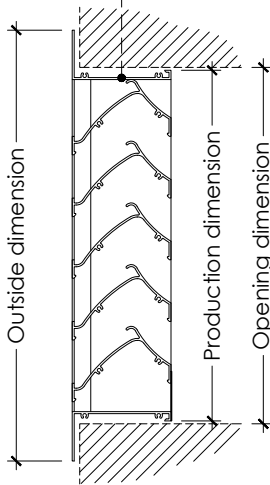
"L" frame (CL)
