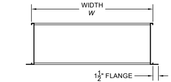
MODEL: ACL845 FRAME: FLANGE FRAME FLANGE-MOUNT (FM)
