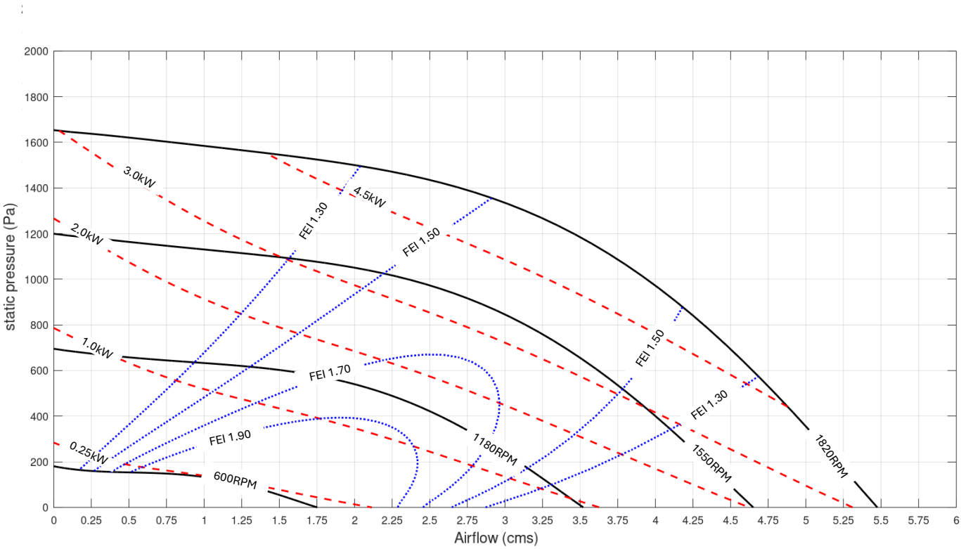
PA-C56-JU56-XXXXX Performance
