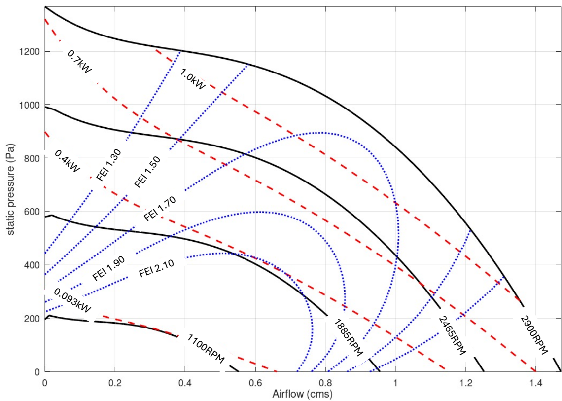
PA-C31-EJ56-XXXXX Performance
