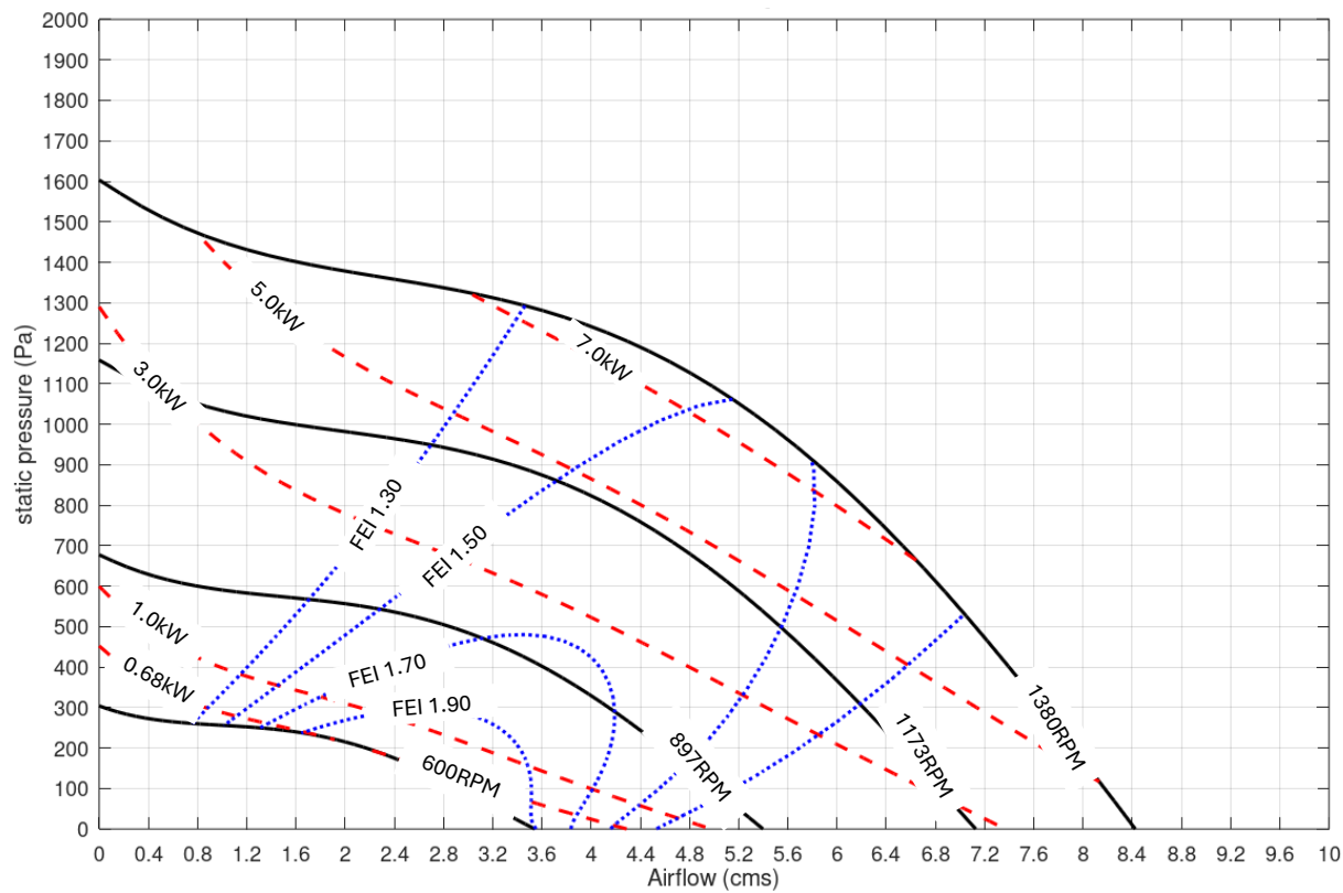
PA-C71-LY56-XXXXX Performance
