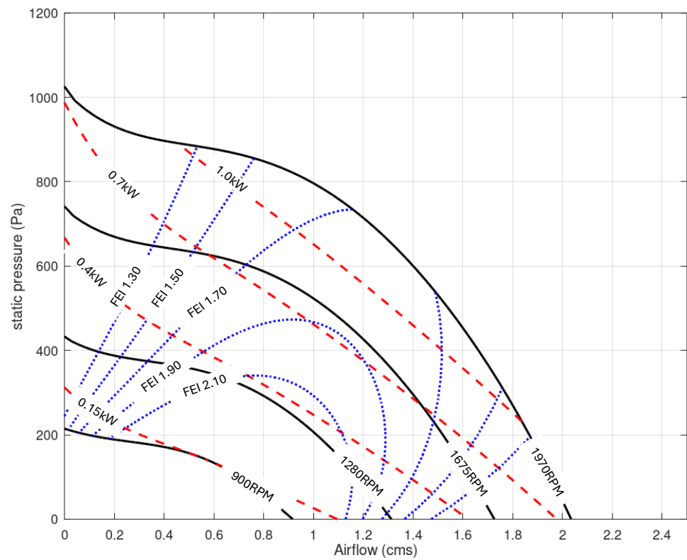
PA-C40-ER56-XXXXXX Performance
