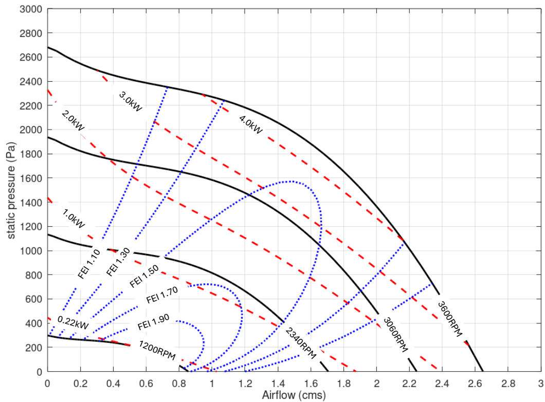
PA-C35-JE56-XXXXX Performance
