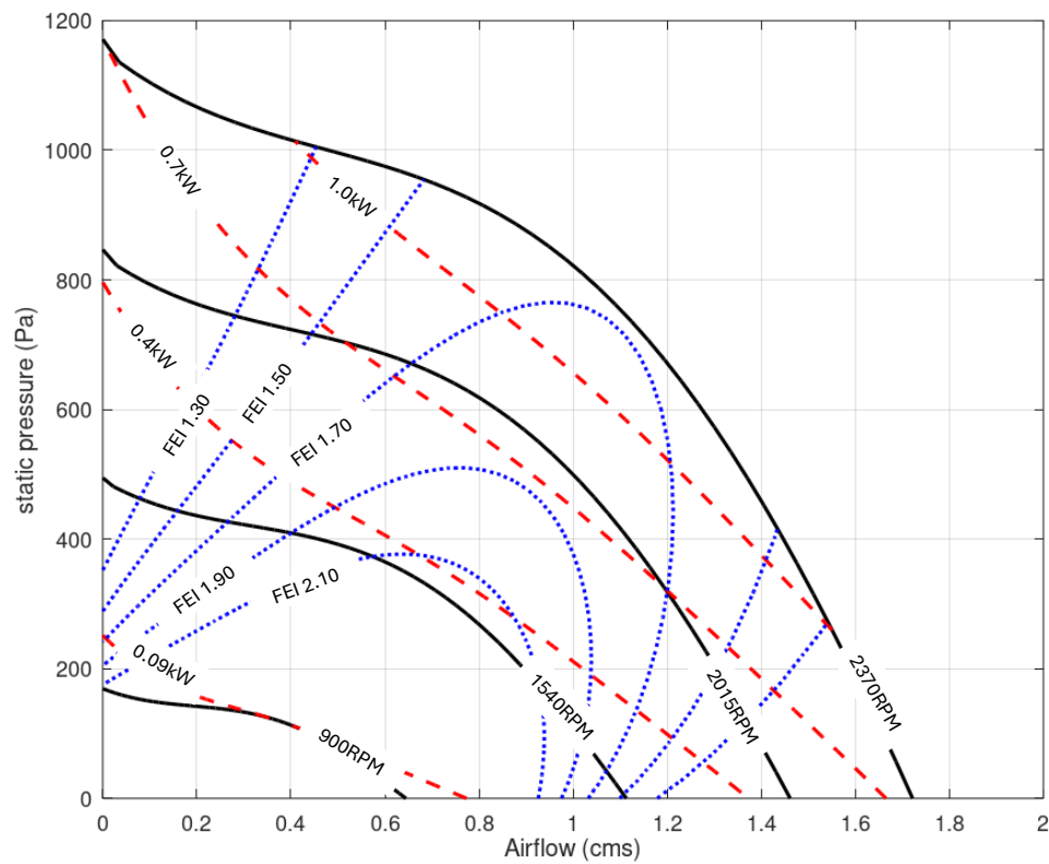
PA-C35-EM56-XXXXX Performance
