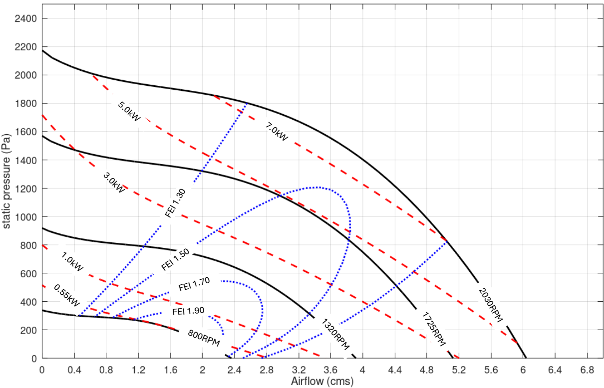
PA-C56-LQ56-XXXXX Performance
