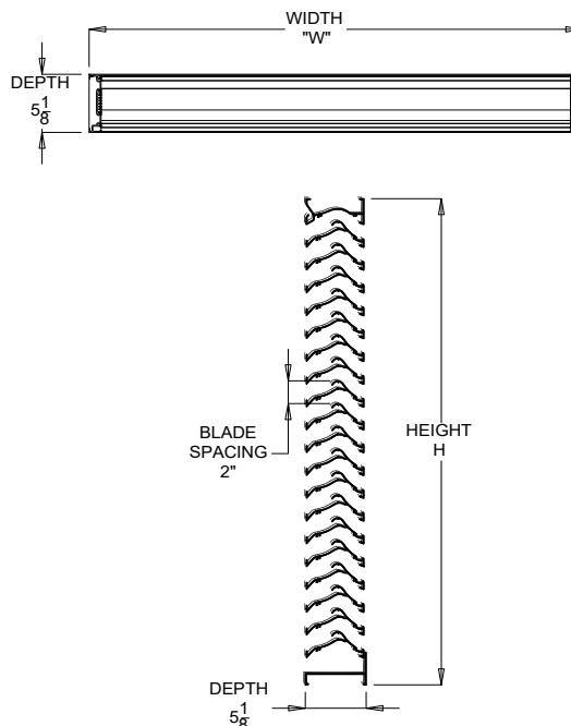
MODEL: 2570H FRAME: CHANNEL FRAME DUCT MOUNT (DM)
