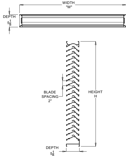
MODEL: 2570H FRAME: CHANNEL FRAME DUCT MOUNT (DM)
