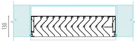
Plan View
