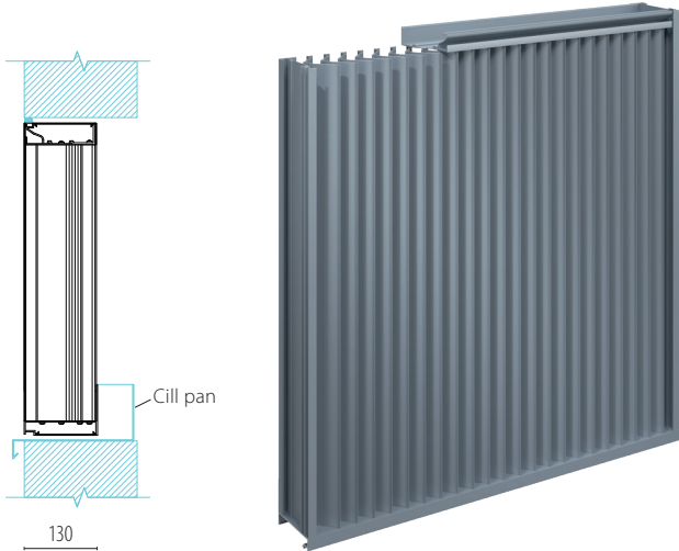
Section View
