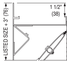
OPT. FLANGED FRAME (FL15 STD.)
