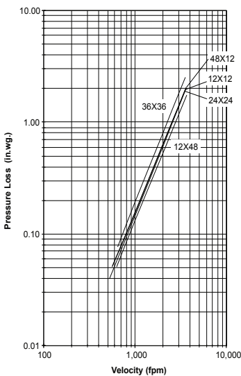
Figure 5.5 Plenum Mount
