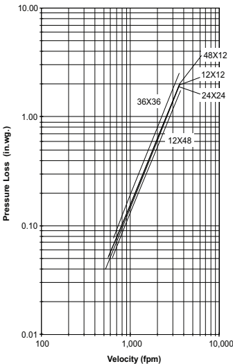
Figure 5.5 Plenum Mount
