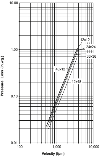
Figure 5.2 — Ducted Inlet
