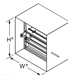
Sleeve (optional)
