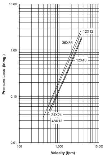
Figure 5.5 Plenum Mount
