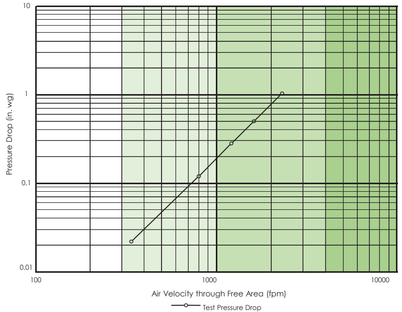
PRESSURE DROP Test Size 48" x 48"
