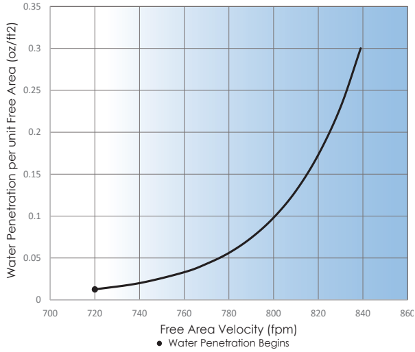
WATER PENETRATION Test Size 48" x 48"
