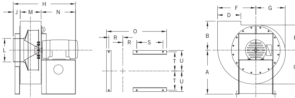
SERIES 20 SIZES 144-364 AND SERIES 30 SIZES 194-364 ARR. 4 – DIMENSIONS [INCHES]
