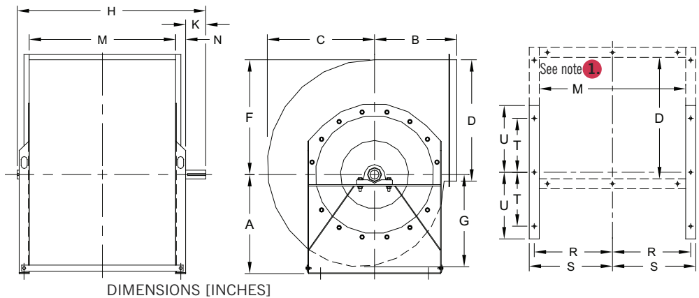
DIMENSIONS [INCHES]
