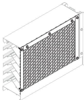
BIRD/INSECT SCREEN (INTERNAL VIEW)
