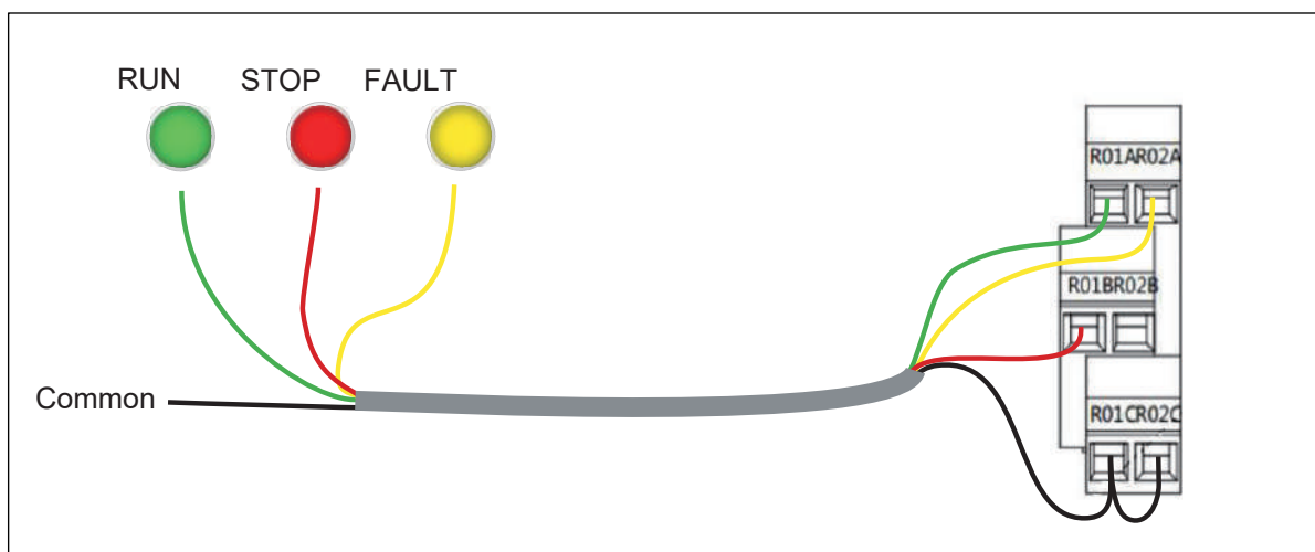
Figure 4 Relay Status
