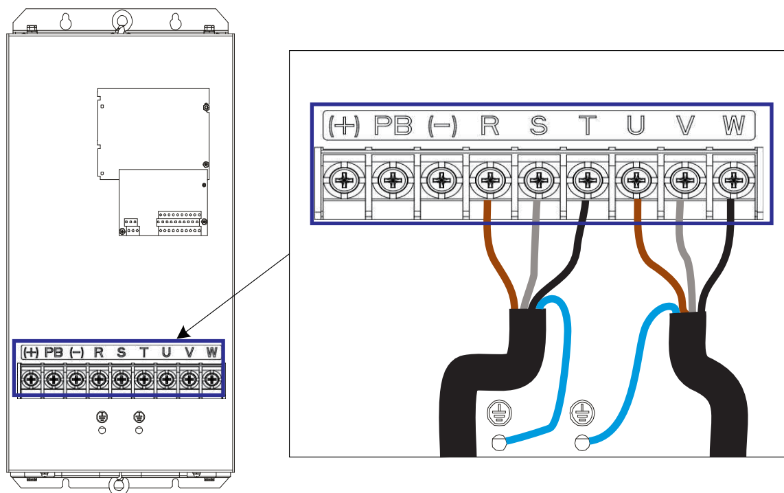
Figure 2 Power Wiring
