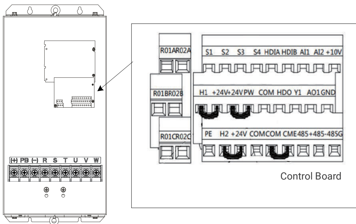
Figure 3 Control Wiring
