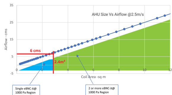
Figure 2 : Typical AHU Models Vs Airflow
