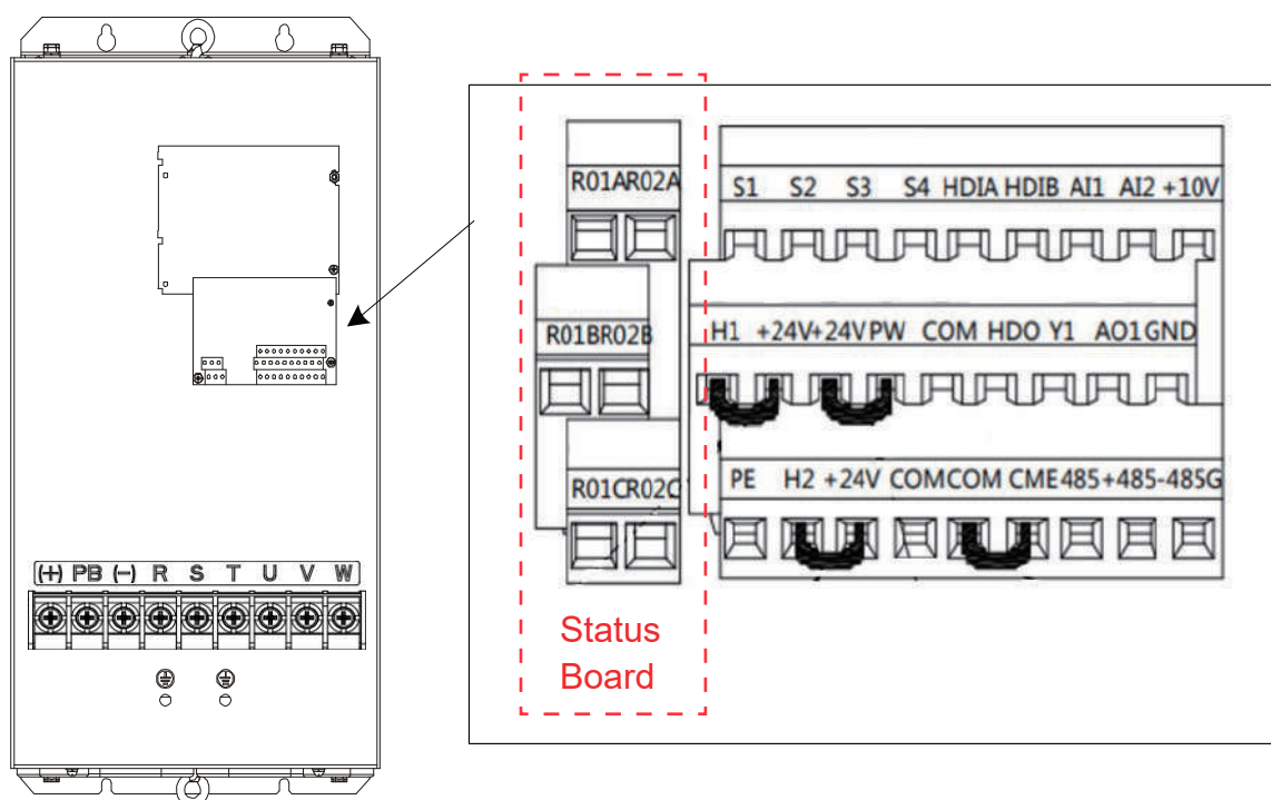
Figure 4 Relay Status
