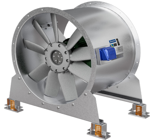
Horizontal Mount
