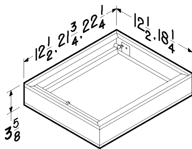
Model RD1 Radiation Damper
