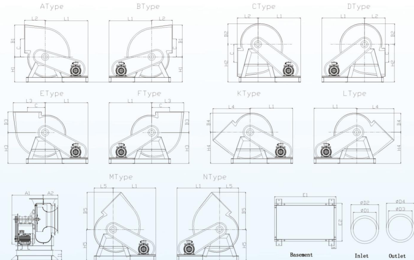
FTY 风机外形尺寸标注
