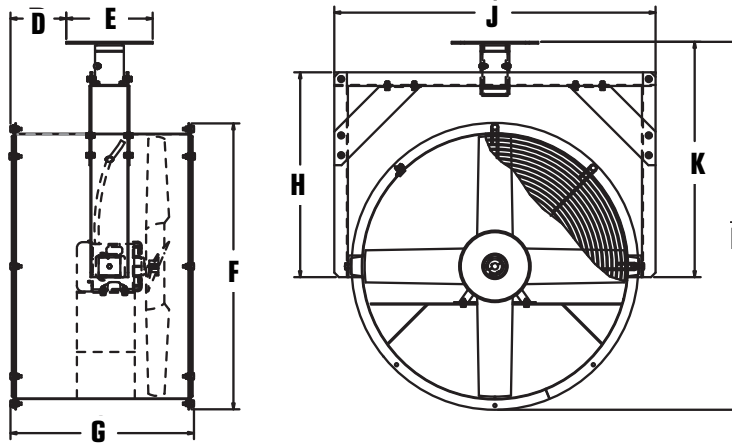
Ceiling Mount
