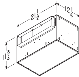
Inline Mount
