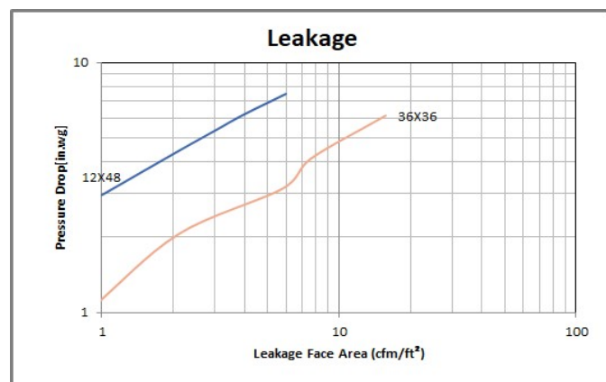
Rating Based on: ANSI/AMCA 500-D-12 Fig 5.4 Alternate
