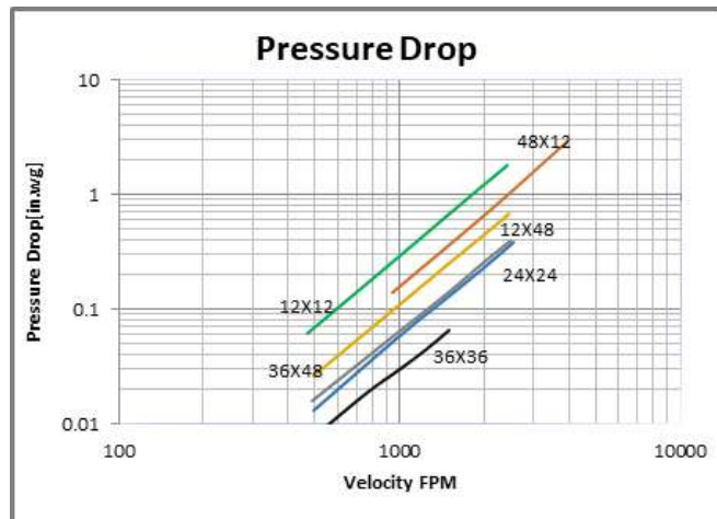
Rating Based on ANSI/AMCA 500-D-18 Fig 5.3
