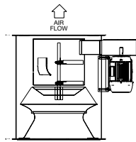
VUI VUO DISCHARGE UP FLOOR OR CEILING MOUNT
