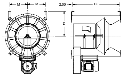
HCH HORIZONTAL CEILING HUNG
