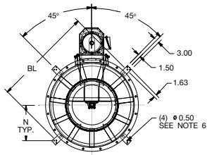
VIEW FROM OUTLET END
