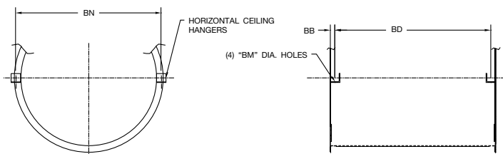
HCH HORIZONTAL CEILING HUNG
