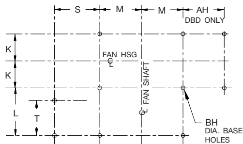
FOUNDATION PLAN (FOR DBD SEE NOTE 1) MOTOR LOCATION 'L' (LEFT) SHOWN
