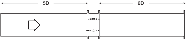
AMCA Figure 5.3
