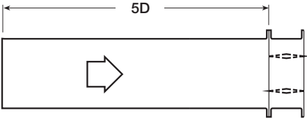
AMCA Figure 5.2
