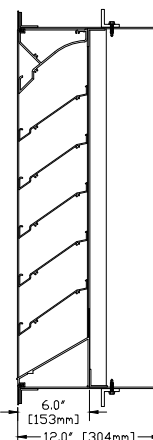
Flange/Sleeve Frame
