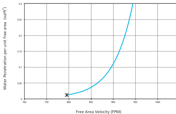
Water Penetration of ACL - 300
