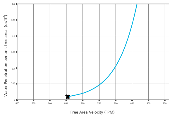
Water Penetration of ACL - 150
