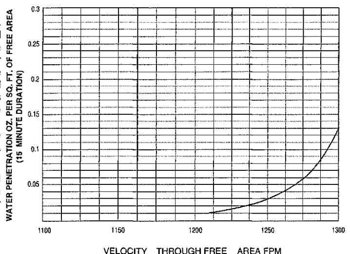
Water Penetration
