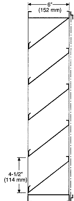
Channel Frame
