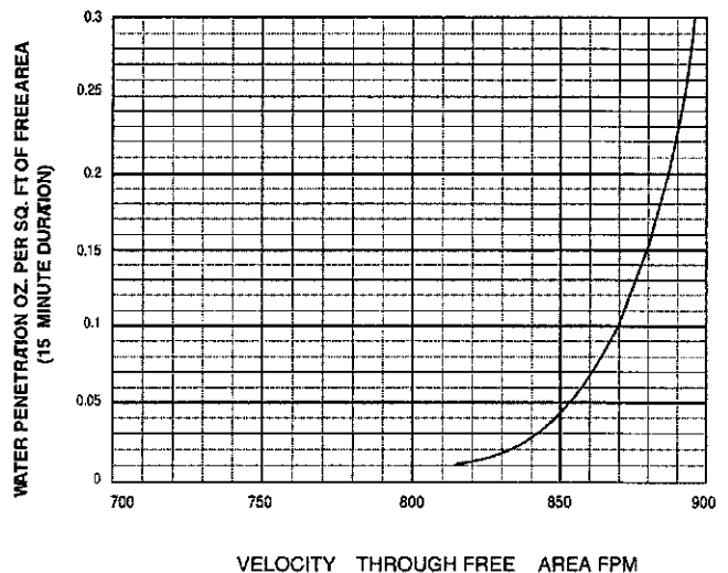
Water Penetration
