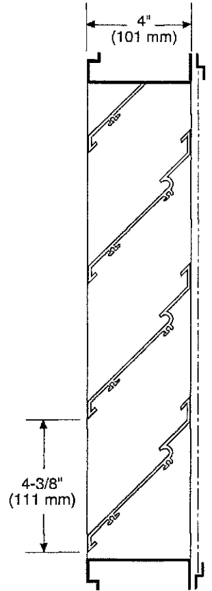
Channel Frame
