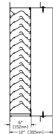
Flange/Sleeve Frame
