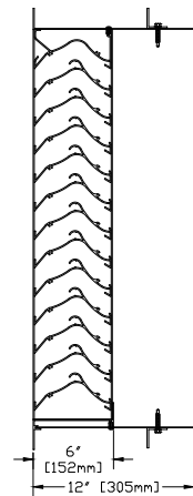
Flange/Sleeve Frame
