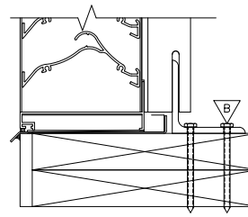
(B) SILL DETAIL AT MULLION
