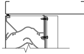
(A1) HEAD DETAIL AT BLADE SUPPORT (SILL DETAIL SIMILAR)
