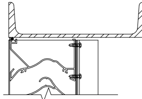
(A1) HEAD DETAIL AT BLADE SUPPORT (SILL DETAIL SIMILAR)
