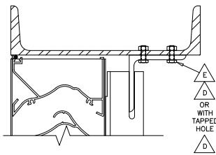
(A) HEAD DETAIL AT MULLION
