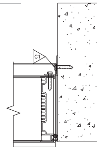
(C) JAMB DETAIL
