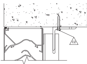
(A) HEAD DETAIL AT MULLION
