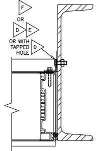
(C) JAMB DETAIL
