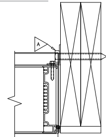
(C) JAMB DETAIL
