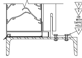
(B) SILL DETAIL AT MULLION
