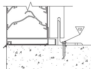
(B) SILL DETAIL AT MULLION
