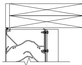
(A1) HEAD DETAIL AT BLADE SUPPORT (SILL DETAIL SIMILAR)
