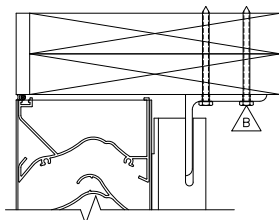
(A) HEAD DETAIL AT MULLION
