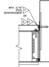
(C) JAMB DETAIL
