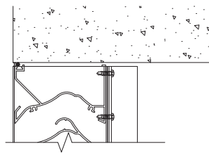
(A1) HEAD DETAIL AT BLADE SUPPORT (SILL DETAIL SIMILAR)
