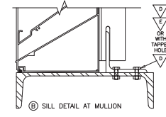
(B) SILL DETAIL AT MULLION
