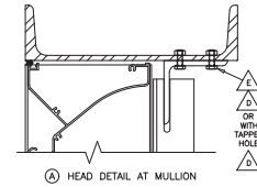
(A) HEAD DETAIL AT MULLION
