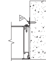
(C) JAMB DETAIL
