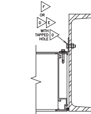
(C) JAMB DETAIL
