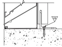
(B) SILL DETAIL AT MULLION
