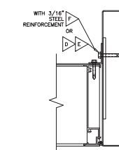
(C) JAMB DETAIL
