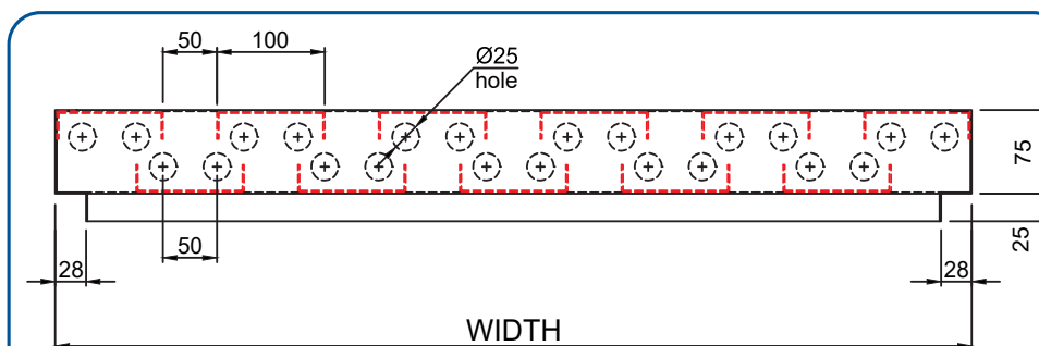
SAND TRAP LOUVERS BOTTOM VIEW DETAILS
