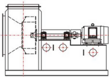
Coupling Drive
