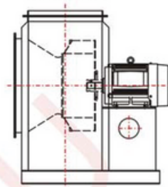
Motor Drive
