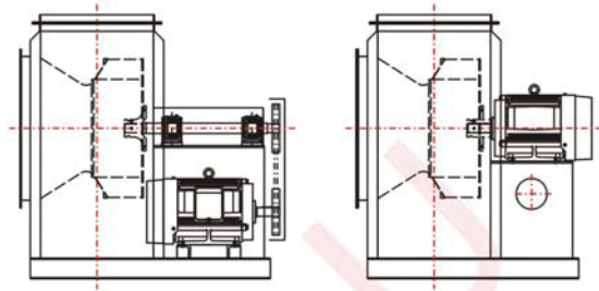
Motor Drive
