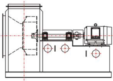
Coupling Drive
