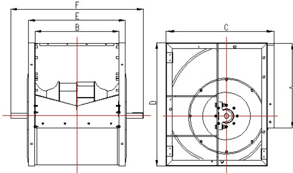
Standard Shape of Backward Double Inlet Centrifugal Fan
