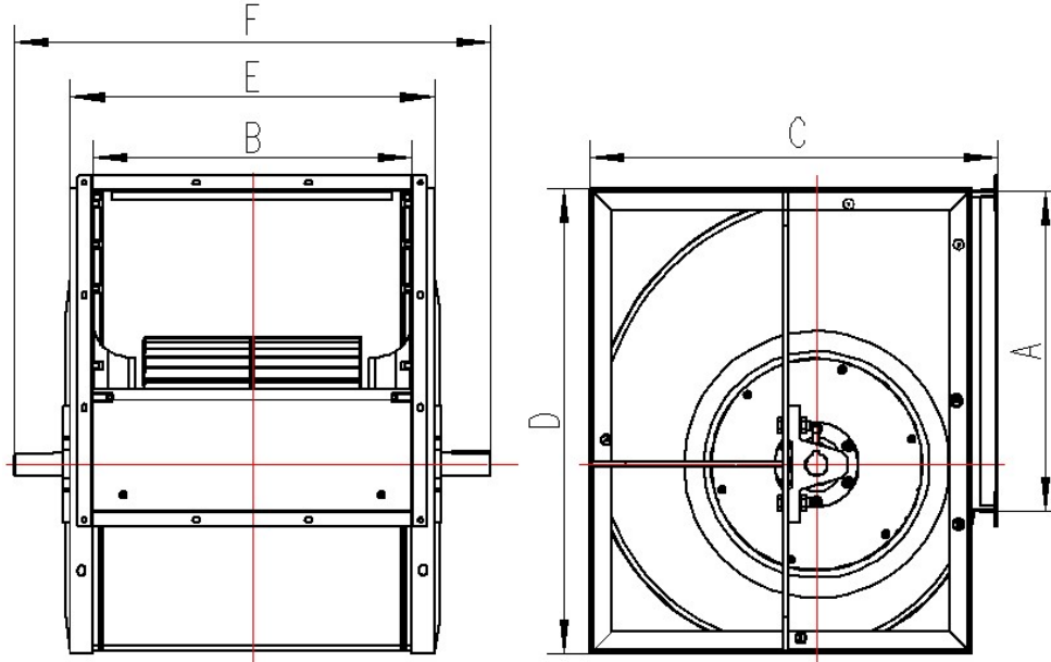
Standard Shape of Forward Double Inlet Centrifugal Fan
