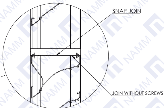
SNAP JOIN INSTALLATION DETAIL
