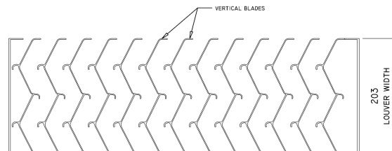
SECTIONAL PLAN
