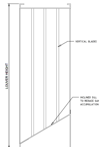
SECTION
