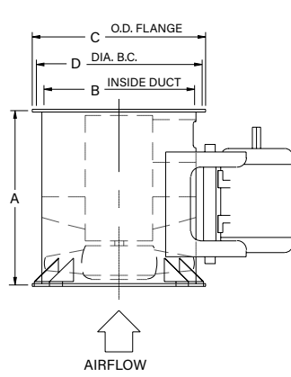
VJBD - ARR. 9 - VERTICAL
