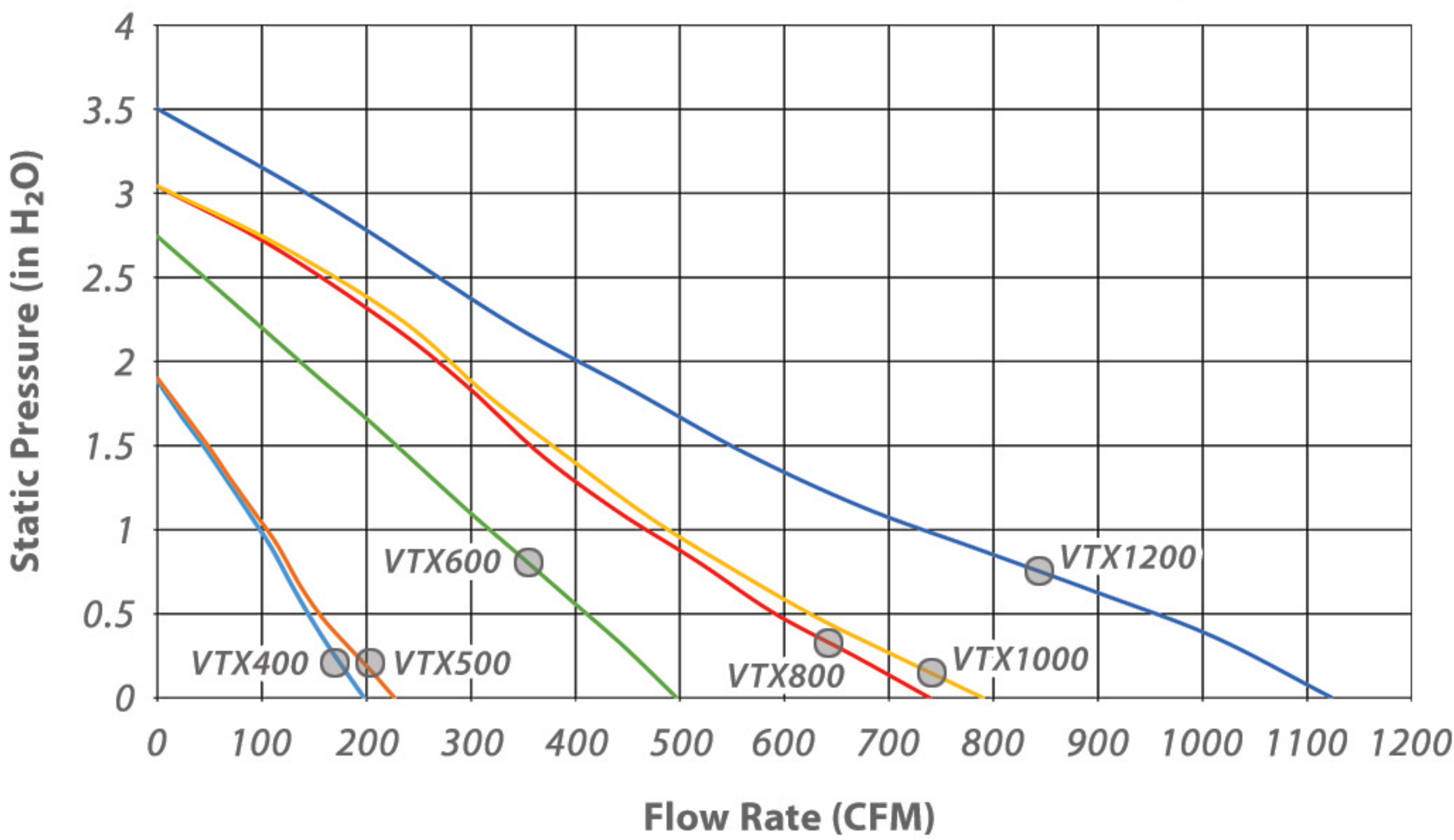
VTX Series Air Performance Graph
