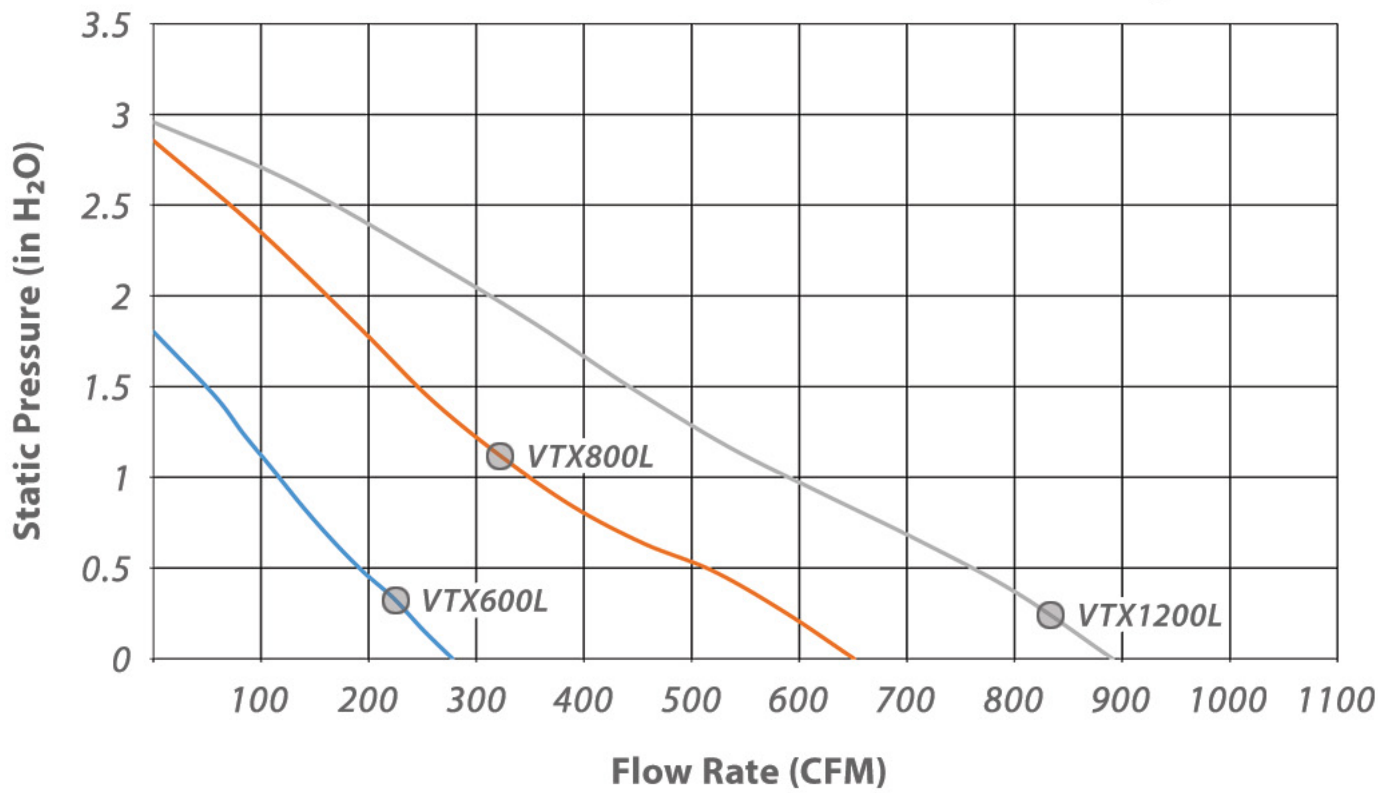
VTX Series "L" Air Performance Graph
