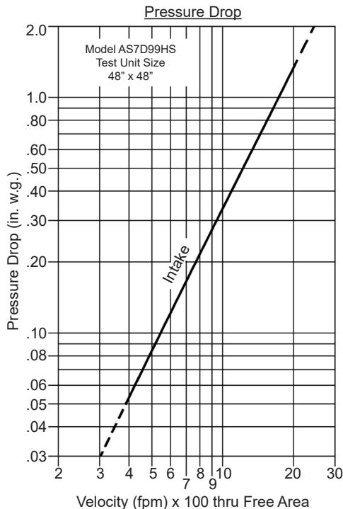
Intake air converted to standard air density. Tested to AMCA Standard 500-L, Figure 5.5.
