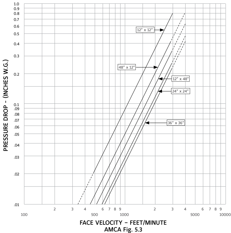
VELOCITY VS. PRESSURE DROP
