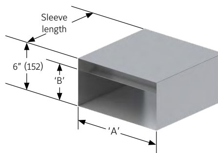
FSD37(LP) STYLE B
