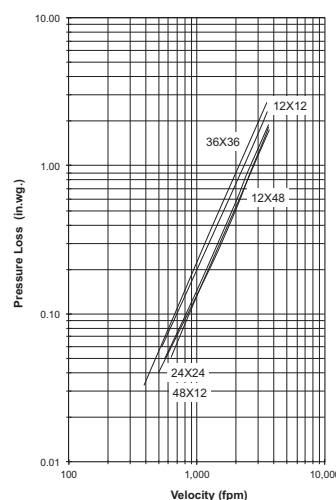
Figure 5.5 Plenum Mount
