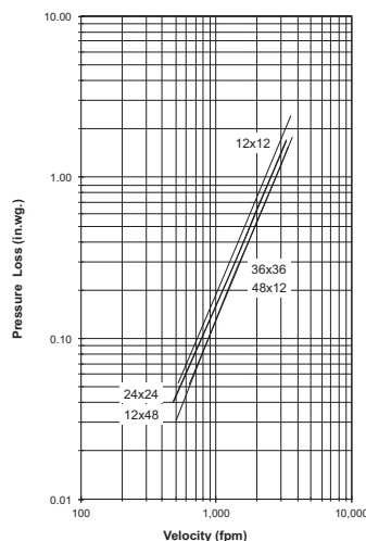
Figure 5.2 — Ducted Inlet
